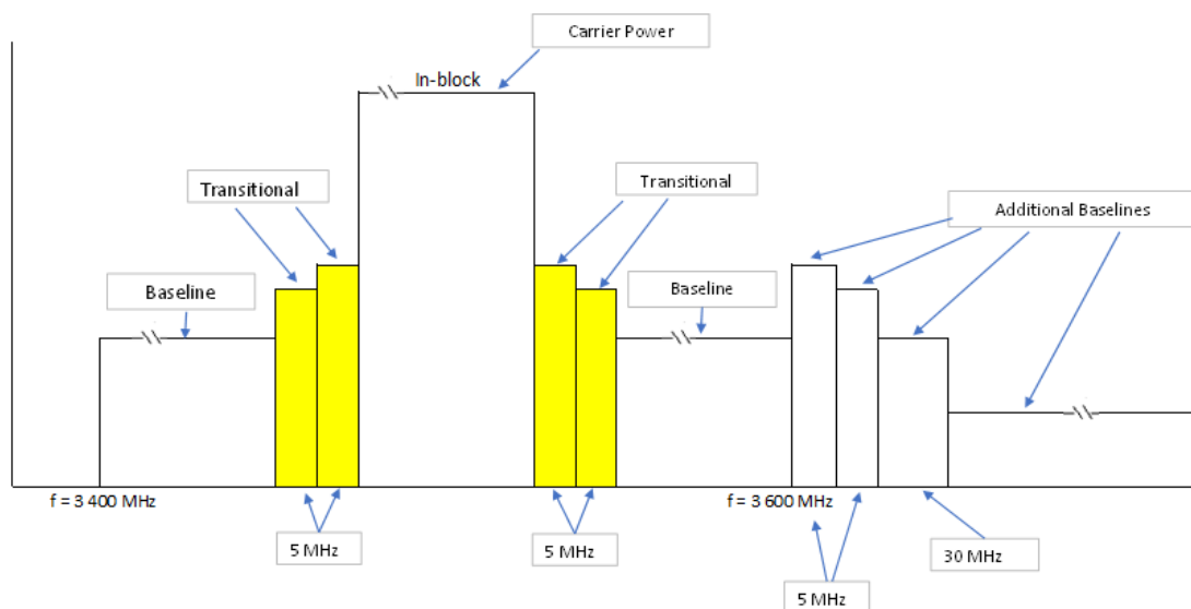
Figure 1 – Power limits for operation within the 3 400 – 3 600 MHz frequency band
